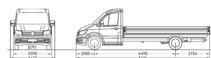
L5SC option plateau
